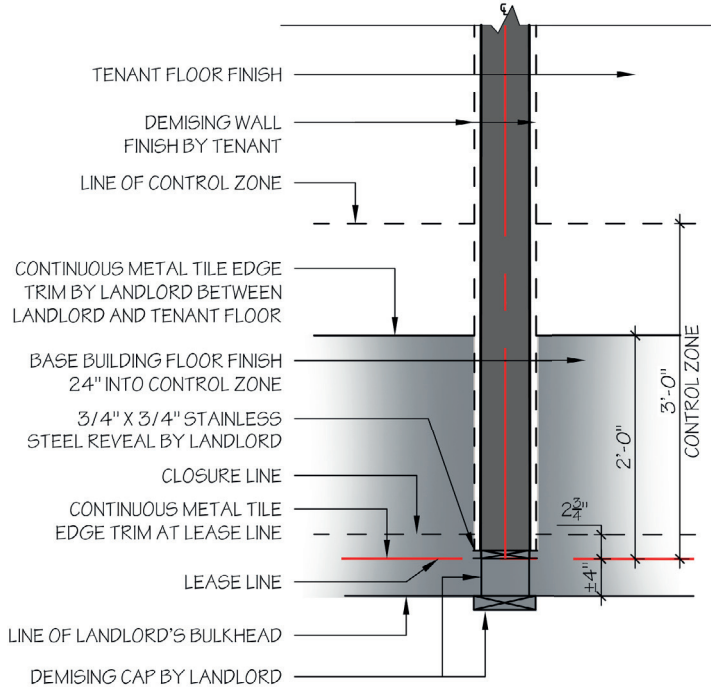
DEMISING CAP CONDITION
