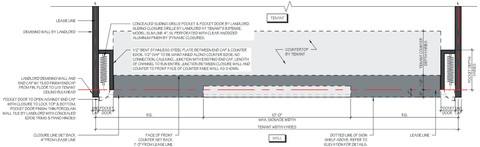
TYPICAL PLAN - FOOD TERRACE STOREFRONT
