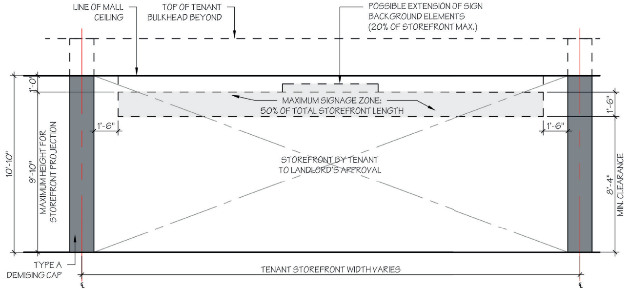
ELEVATION - TYPICAL STOREFRONT
