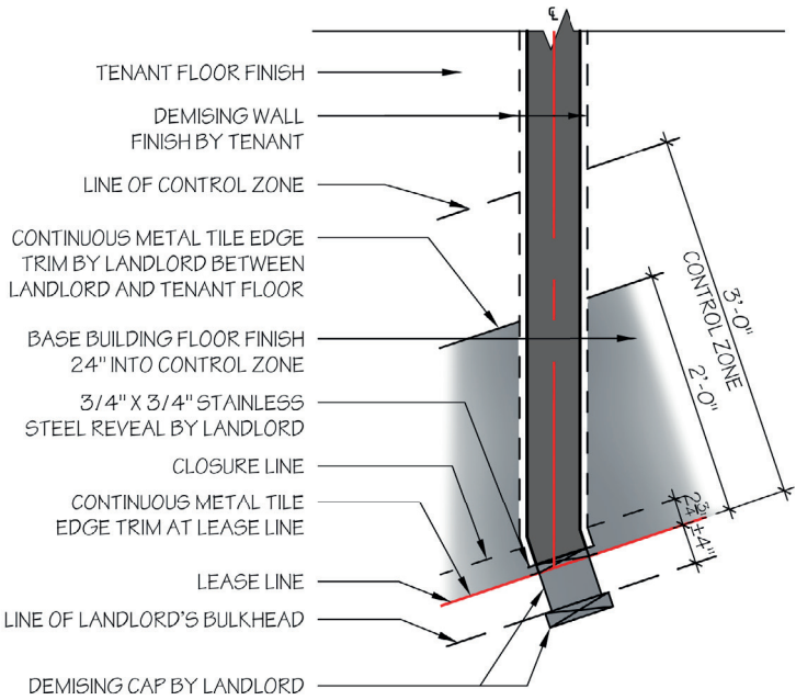
DEMISING CAP CONDITION AT ANGLED LEASE LINE
