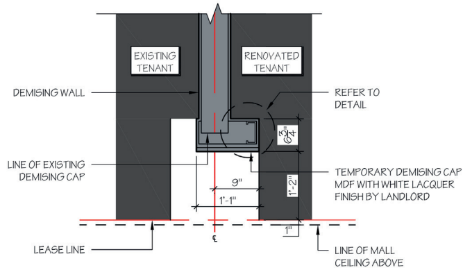
TYPE A1 - INTERIM DEMISING CAP (BY LANDLORD)
