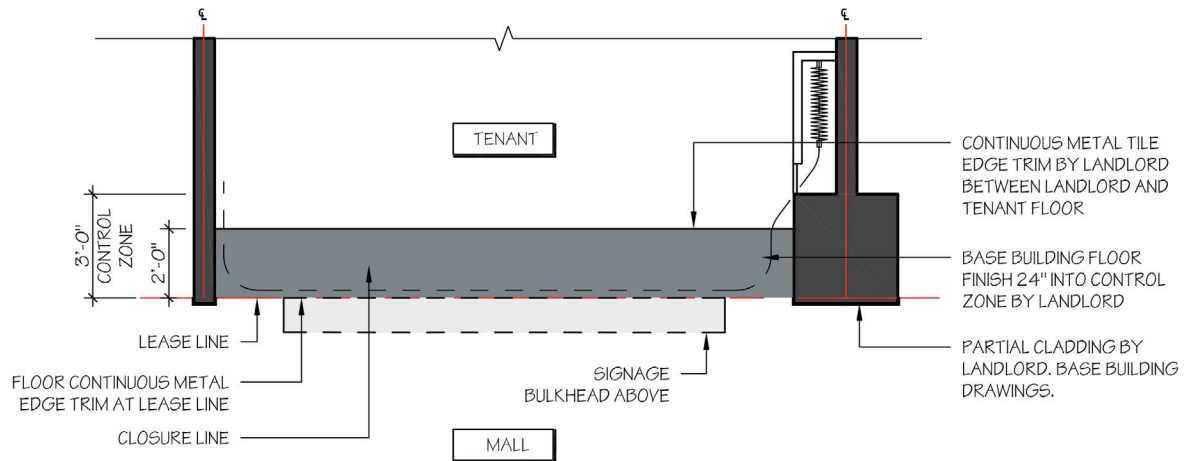
PLAN - TYPICAL CONDITION B
