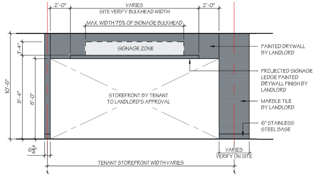
ELEVATION - TYPICAL CONDITION B
