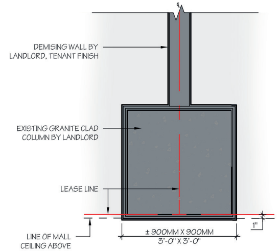
TYPE C - DEMISING COLUMN
