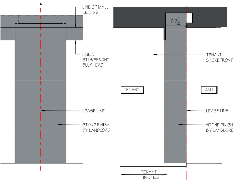
DEMISING CONDITION A
