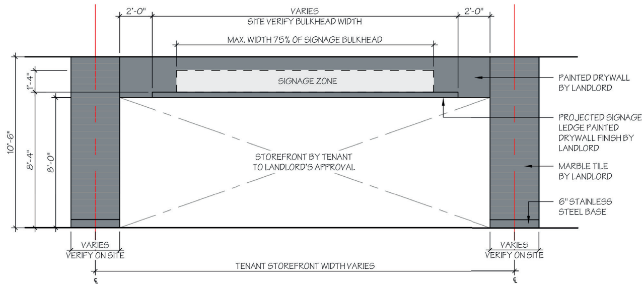
ELEVATION - TYPICAL CONDITION A
