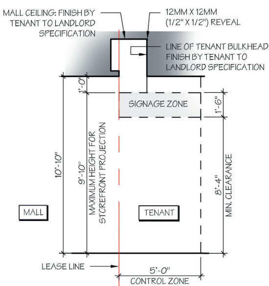
SECTION - TYPICAL STOREFRONT
