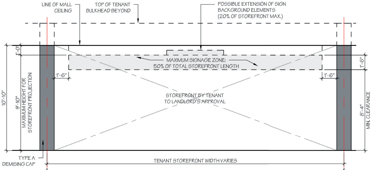
ELEVATION - TYPICAL STOREFRONT
