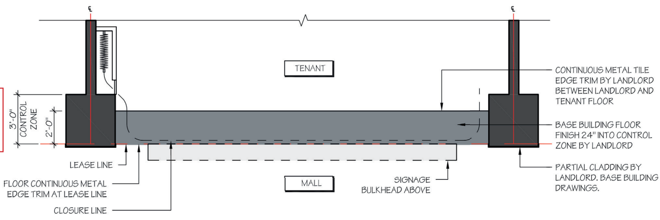
PLAN - TYPICAL CONDITION A
