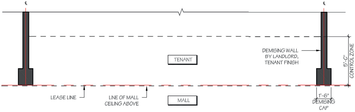
PLAN - TYPICAL STOREFRONT
